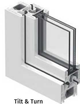
Tilt & Turn
