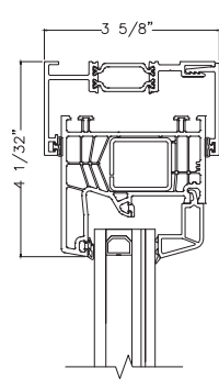
Head Receptor
